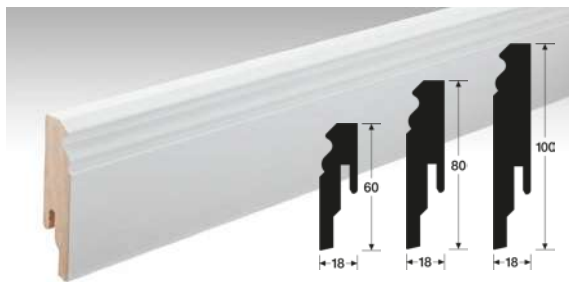
Hamburg skirting board HSL 60 | 80 | 100 (white) 18 x 60 x 2380 mm 18 x 80 x 2380 mm 18 x 100 x 2380 mm
