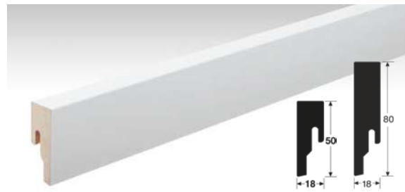
Design skirting board DSL 50 | 80 (white) 18 x 50 x 2380 mm 18 x 80 x 2380 mm
